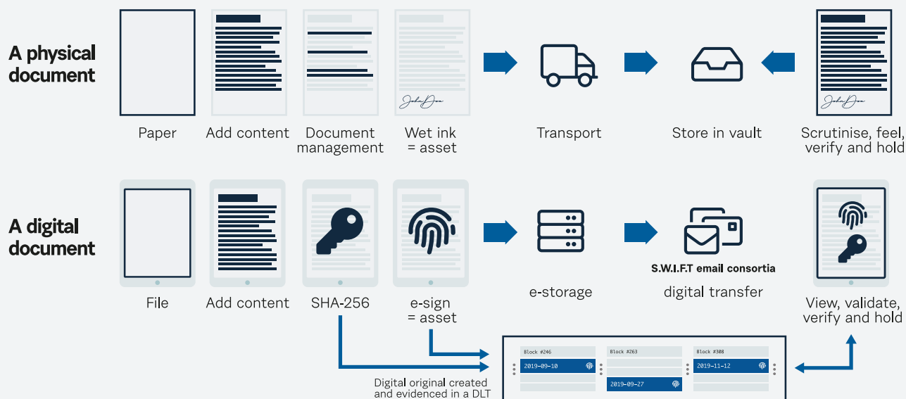
Fig. 1 | trace:original, how it compares to physical paper documents
